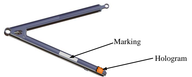
F.41.15.004 Rear pushrod
