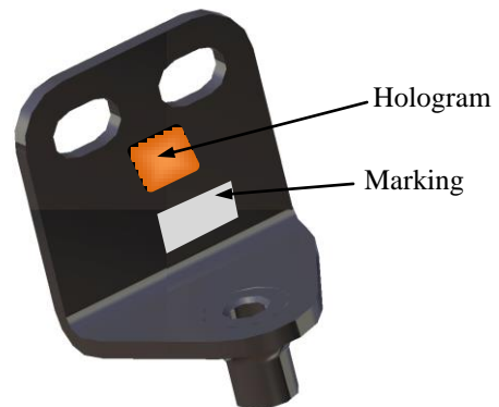
F.41.21.056 Bracket, extinguisher retainer
