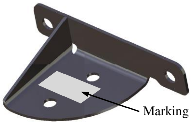
F.41.21.025 Bracket, throttle pedal sensor
