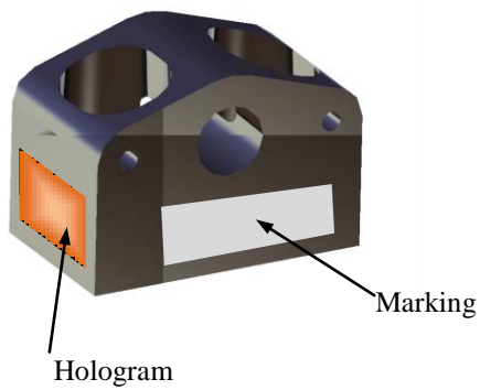
F.41.19.018 Bracket, front crashbox
