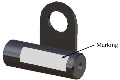
F.41.21.058 Stop sleeve bracket
