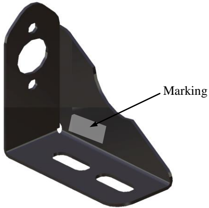
F.41.26.027 Bracket, front cover
